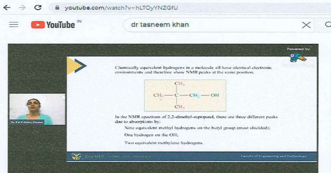
NMR SPECTROSCOPY
