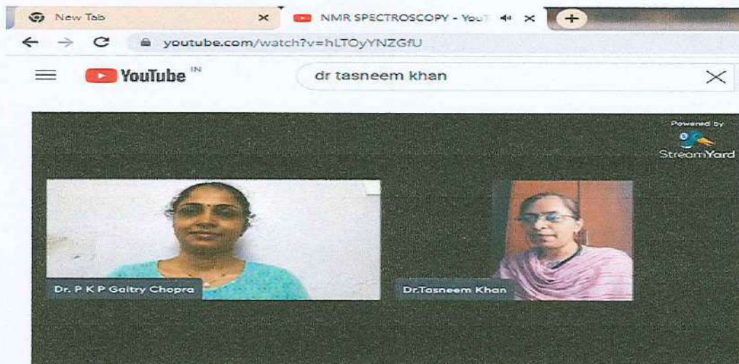
NMR SPECTROSCOPY
